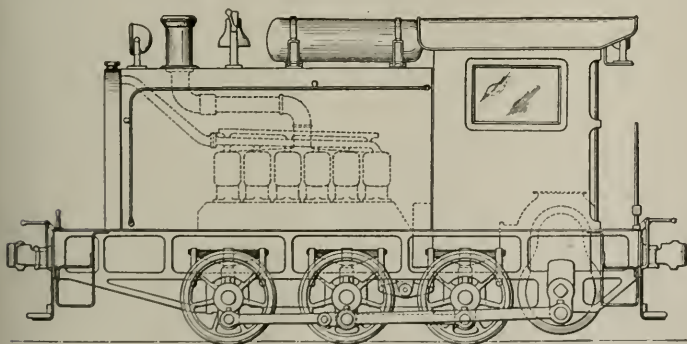
GENERAL ARRANGEMENT OF SIX-COUPLED, 15 AND 25 TON LOCOMOTIVE.
